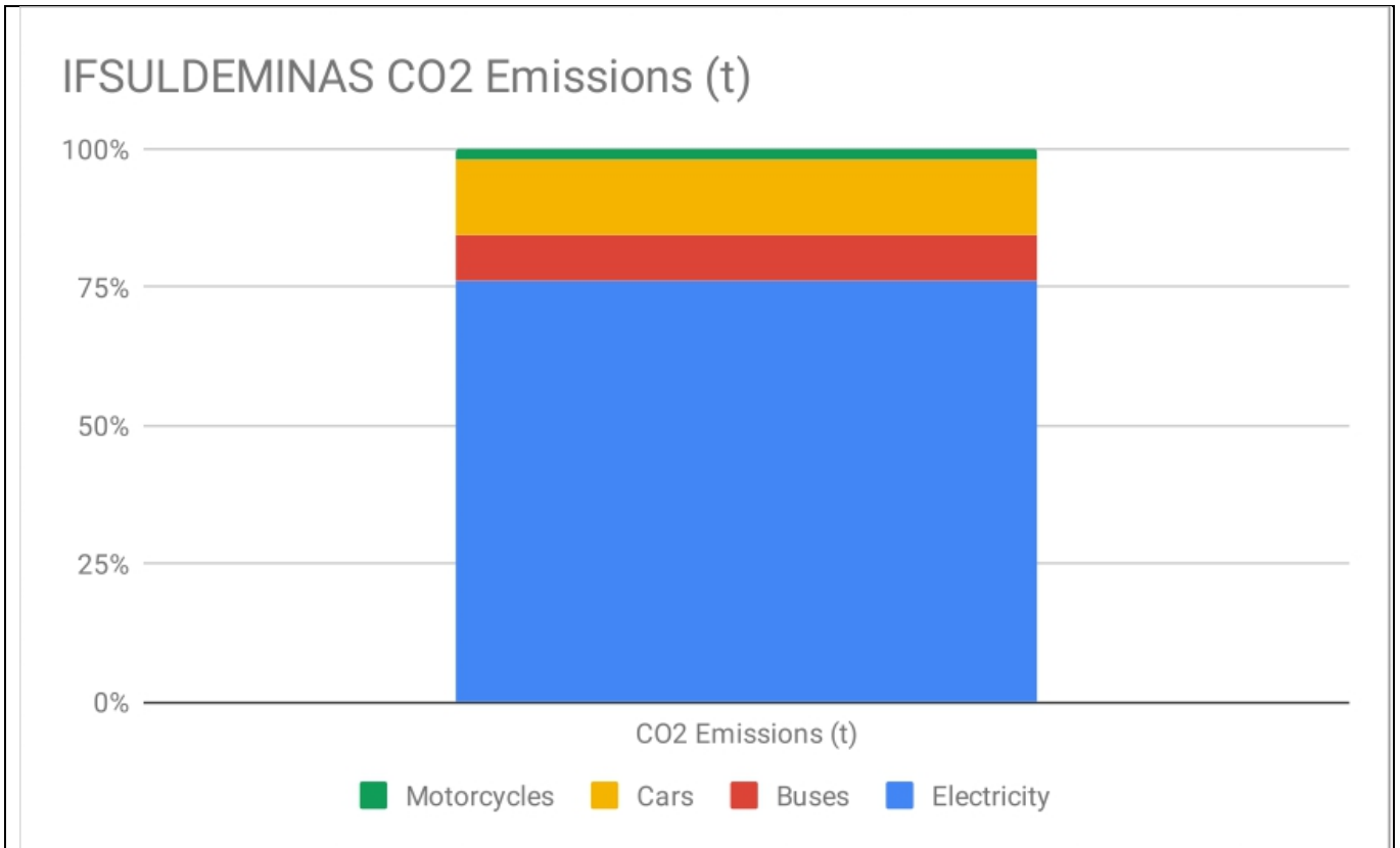
Graphic 1: IFSULDEMINAS CO 2 emissions in the last 12 months.
